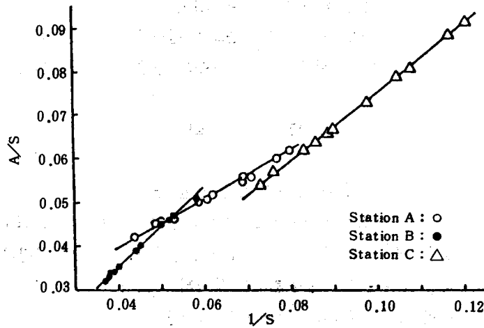
Fig 5. Relation between 1/S and A/S in the middle layer water of observation station A, B and C. S : Salinity, A : Alkalinity
