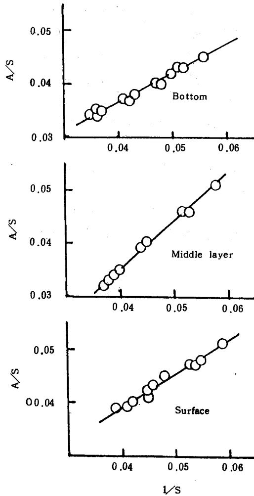
Fig 3. Relation between 1/S and A/S in the water of observation station(B) S: Salinity, A: Alkalinity
