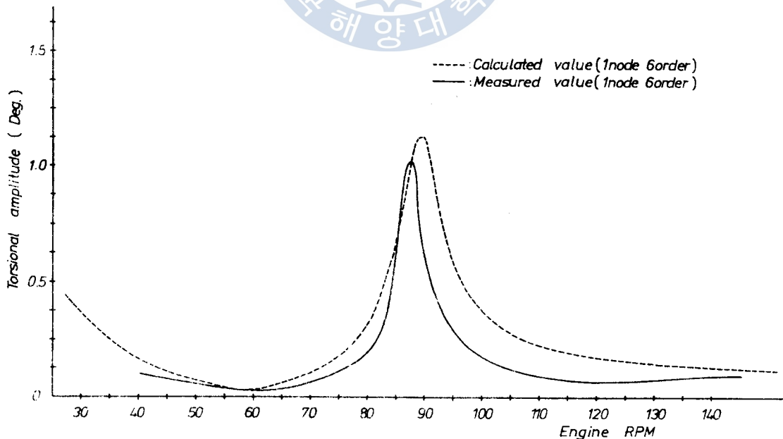
Fig. 2. Amplitude of torsional vibration at crankshaft fore-end(6RND68)
