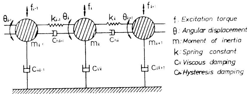
Fig. 1. The modeling of the forced torsional vibration with damping
