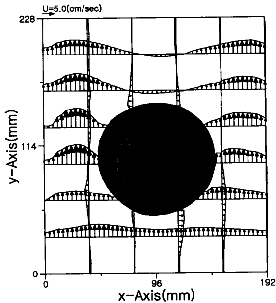
Fig.2 Time-mean velocity profile around a cooled tube ; U_i = 0.05\text{m/s} , T_w = -20.0^\circ\text{C} , Q_{\text{air}} = 30 \text{ l/min}
