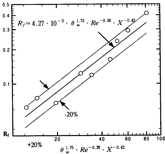
Fig.12 Dimensionless frozen quantity
