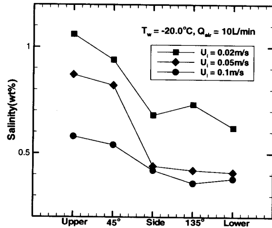
Fig.6 Salt concentration of external frozen layer in the steady state ; Q_{air}=10 \text{ l / min} , T_w=-20^\circ\text{C}
