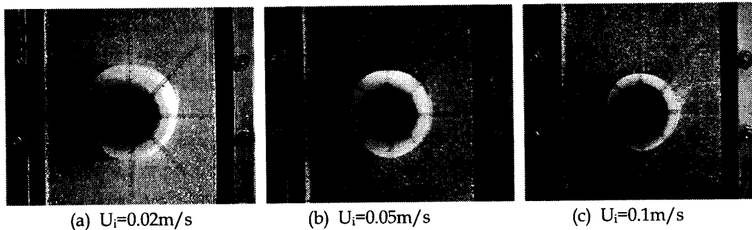
Fig.4 Effect of fluid velocity on freezing behavior ; Q_{\text{air}} = 10 \text{ l/min} , T_w = -20^\circ\text{C}
