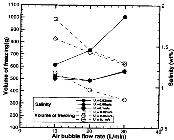
Fig.9 Mean salt concentration of frozen layer ; T_w = -20^\circ\text{C}
