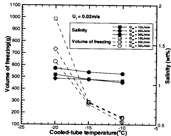
Fig.11 Mean salt concentration of frozen layer ; U_i = 0.02\text{m/s}
