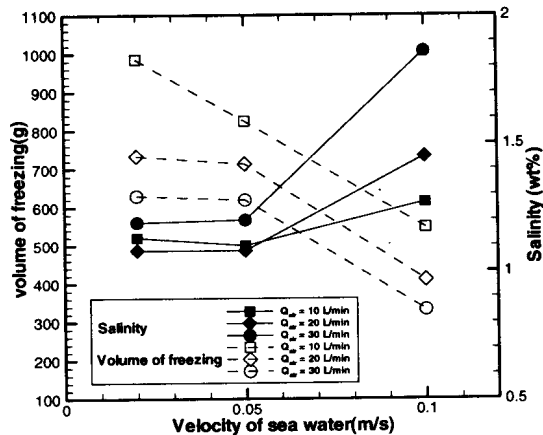
Fig.7 Mean salt concentration of frozen layer ; T_w = -20^\circ\text{C}
