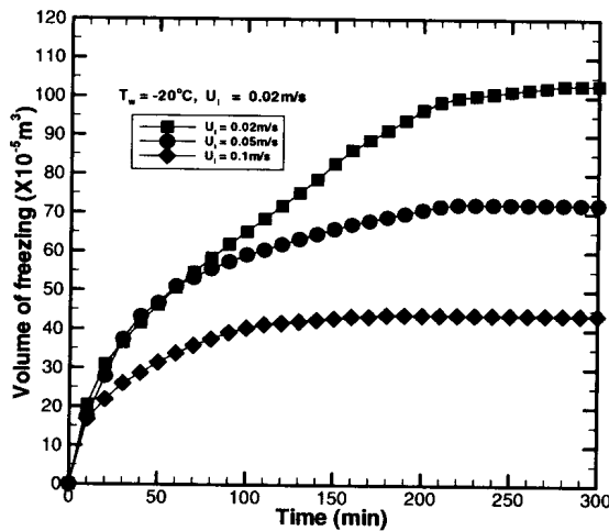
Fig.5 Effect of fluid velocity on volume of freezing; Q_{air}=10 \text{ l / min} , T_w=-20^\circ\text{C}
