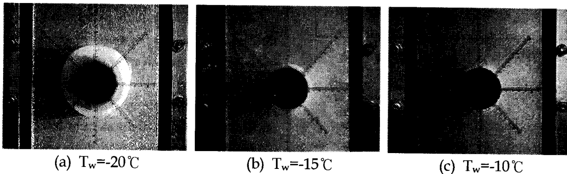
Fig.10 Effect of cooled-tube temperature on freezing behavior ; Q_{\text{air}} = 10 \text{ l/min} , U_i = 0.02\text{m/s}
