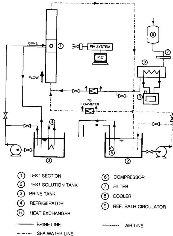
Fig.1 Schematic of experimental apparatus
