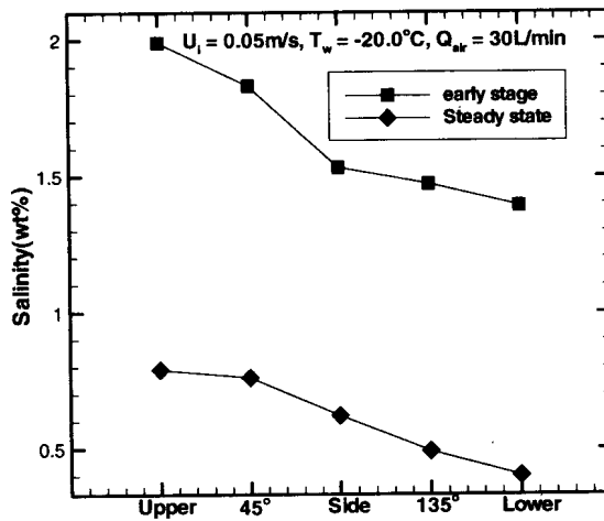
Fig.3 Salinity distribution of frozen layer ; U_i = 0.05\text{m/s} , T_w = -20.0^\circ\text{C} , Q_{\text{air}} = 30 \text{ l/min}
