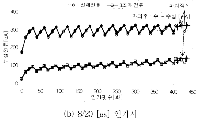
Fig. 6 Changes in leakage current by overtime lightning impulse current
