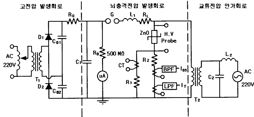
Fig. 1 Configuration of the experimental system
