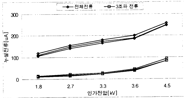
Fig. 3 Changes in leakage current caused by applied A.C voltage
