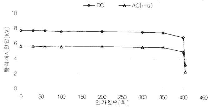
Fig. 5 Changes in reference voltage by overtime lightning impulse current
