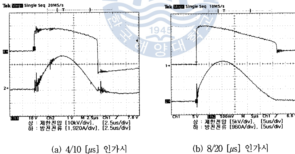
Fig. 2 Typical waveforms to lightning impulse current
