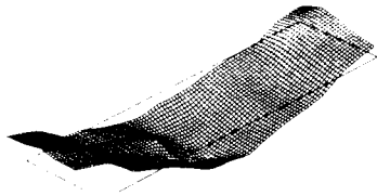
Fig. 10 First bending mode (15.96 Hz)
