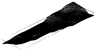
Fig. 11 First torsional mode (23.69 Hz)
