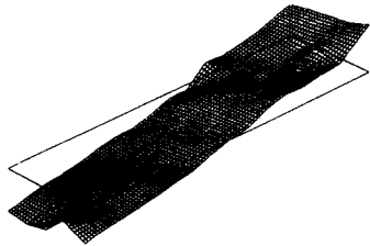
Fig. 7 Heaving mode (10.0 Hz)
