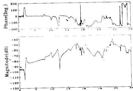
— : Measured acceleration --- : Synthesized acceleration by proportional viscous damping system Fig.5 Measured and synthesized acceleration
