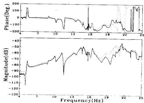
— : Measured accelerance --- : Synthesized accelerance by general viscous damping system Fig.4 Measured and synthesized accelerance
