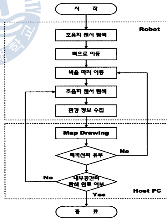
Fig. 7 Flowchart of the map building algorithm
