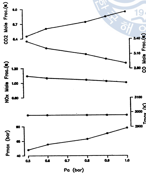
Fig.3-9 Calculated Results of Exhaust Emissions versus Charge Air Pressure at Constant Equivalence Ratio
