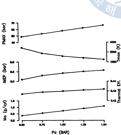
Fig.3-7 Calculated Results of Exhaust Emissions Various Charging Air Pressure at Constant Fuel Amount (IC=-140deg)
