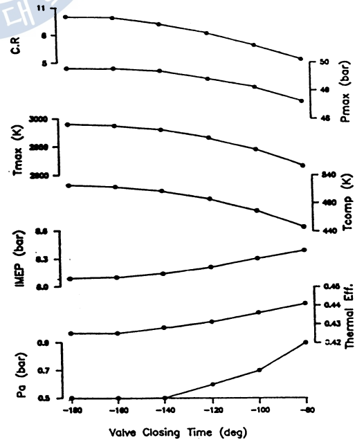
Fig.3-2 Calculated Results of Exhaust Emissions versus Closing Time(T1=Constant)
