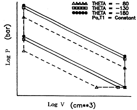
Fig.2-1 Comparisons of P-V Diagram for Miller Cycle (Pa=Constant)
