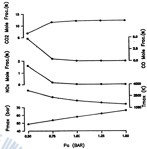
Fig.3-6 Calculated Results versus Various Charging Air Pressure at Constant Fuel Amount (IC=-140deg)
