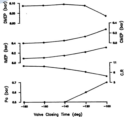
Fig.3-10 Calculated Results versus Valve Closing Time(Phi=1.0)
