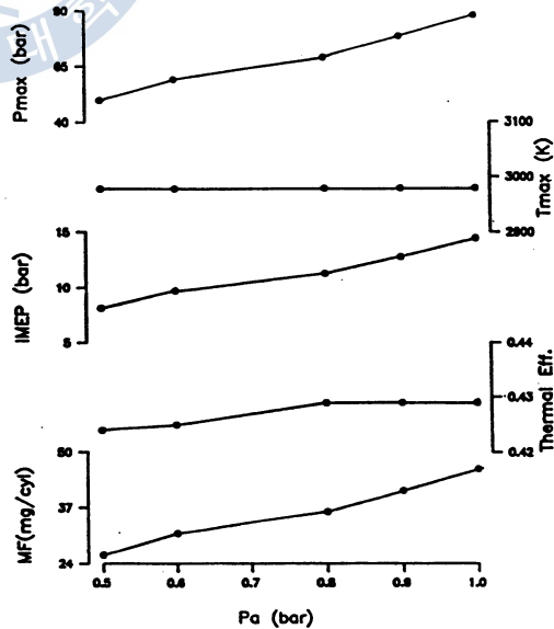
Fig.3-8 Calculated Results versus Charge Air Pressure at Constant Equivalence Ratio
