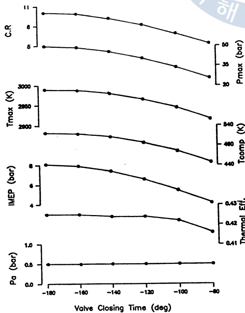
Fig.3-1 Calculated Results versus Various Valve Closing Time(T1=Constant)
