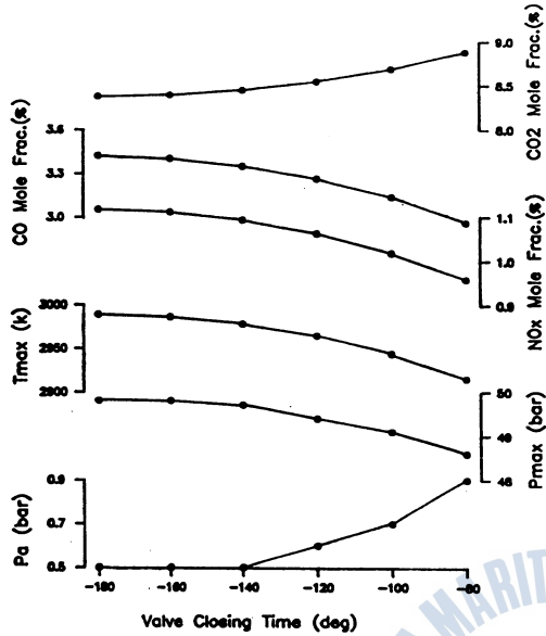
Fig.3-5 Calculated Results of Exhaust Emissions versus Closing Time (T1=Constant)
