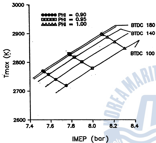
Fig.3-11 Relations between Tmax and IMEP versus Variable Closing Time
