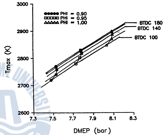
Fig.3-12 Relations between Tmax and DMEP versus Variable Closing Time
