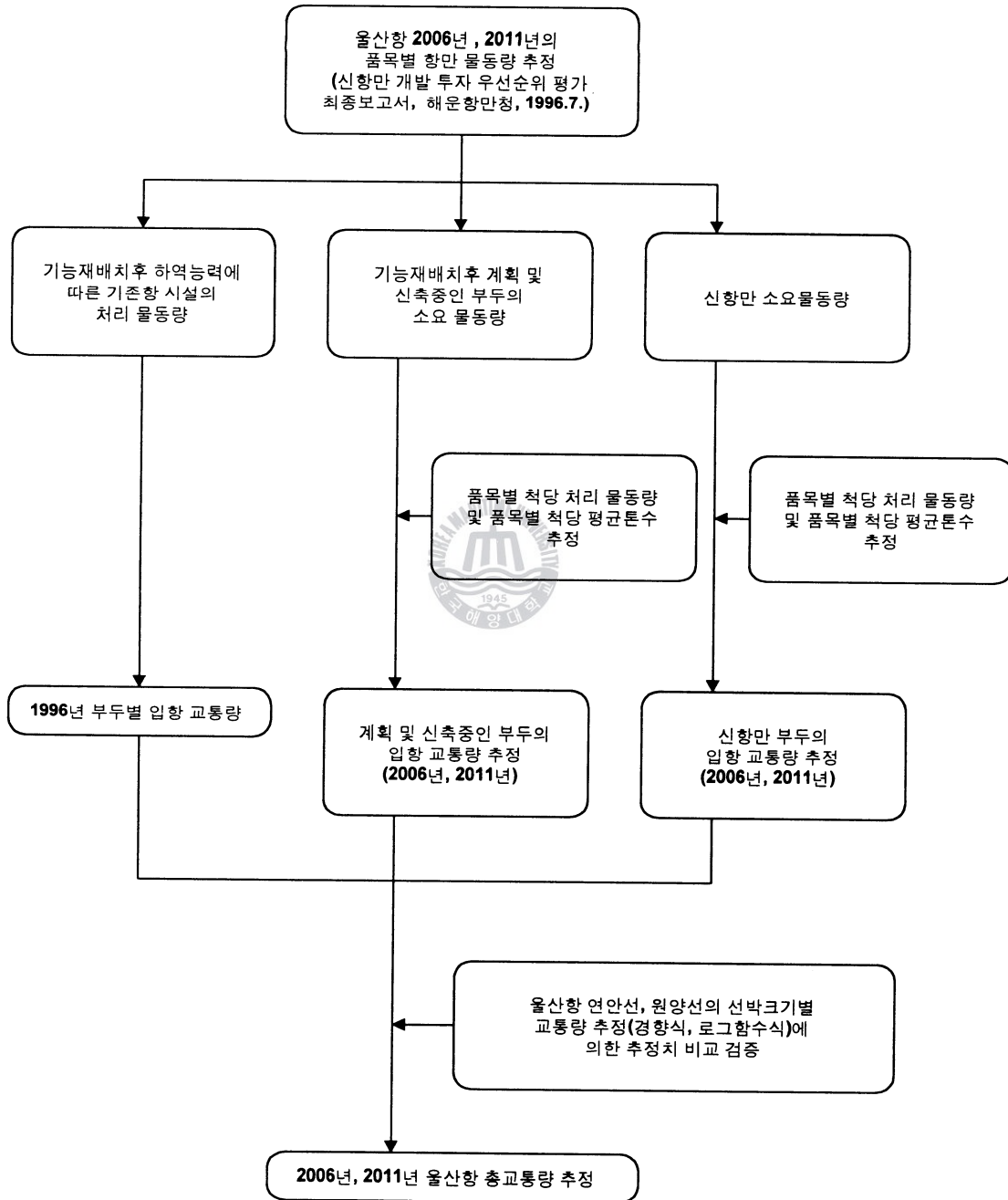
Fig. 1 Flow Chart to estimate the Ulsan's Traffic Volumes (2006, 2011)
