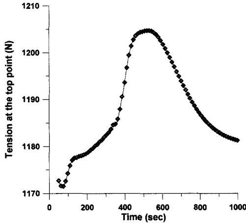
Fig. 7. Tension variation at the top point ( V_f=3.5\text{m/s} , W_{tf}=900\text{N} ).
