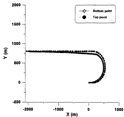
Fig. 6. Trajectory of bottom and top points ( V_t=3.5 m/s, W_{tf}=900 N).
