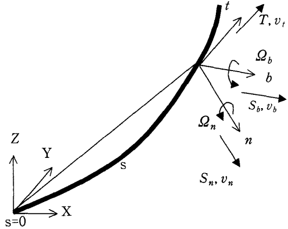
Fig. 1. Coordinate systems.
