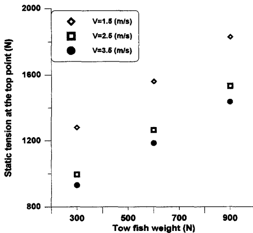
Fig. 3. Static tension for different towing speeds at the top point.
