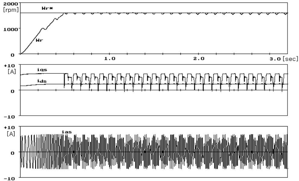
(b) Proposed adaptive controller
