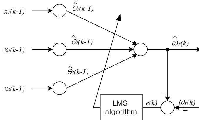
Fig. 4-3 The model of a plant neural estimator
