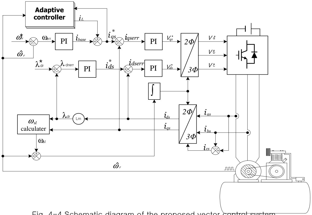
Fig. 4-4 Schematic diagram of the proposed vector control system
